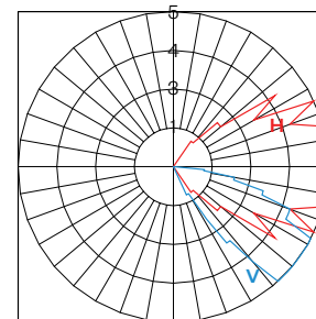
Polar Graph (PRCL8.L40)
