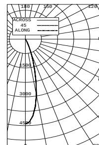
FLOOD DISTRIBUTION LTL # 818201
