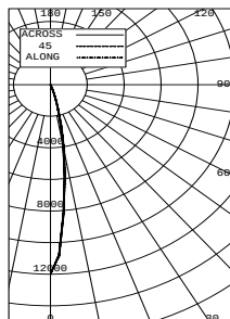
SPOT DISTRIBUTION LTL # 818198
