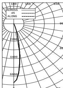
NARROW FLOOD DISTRIBUTION LTL # 818199
