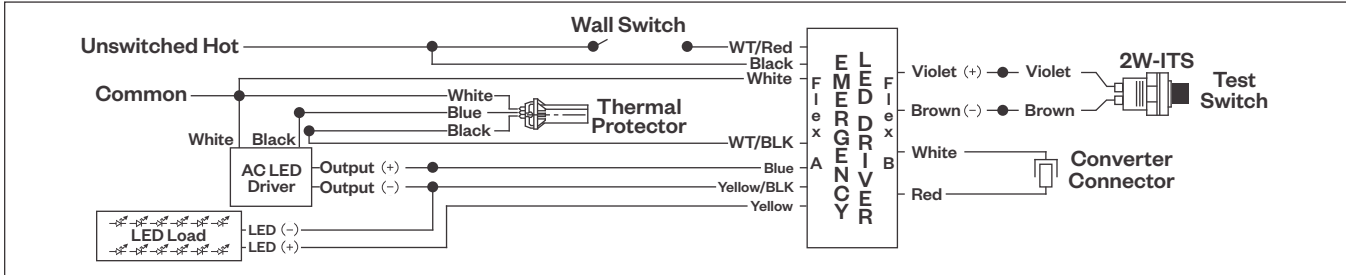
Wiring Diagram
