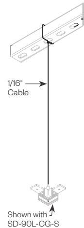
Wrap Around Aircraft Cable only (when suspending to L, T, X Connector with cable gripper)
