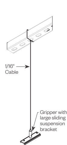
Wrap Around (with sliding suspension bracket)
