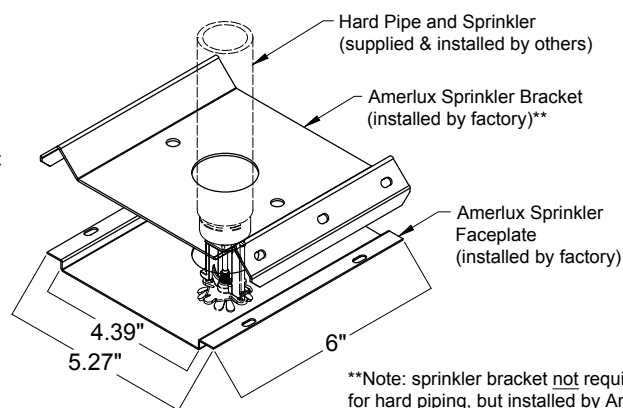
Type: SPR RECESSED HARD PIPING DETAIL
