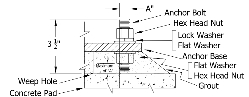
Bolt Projection for Double Nut Application: 3 1/2"
